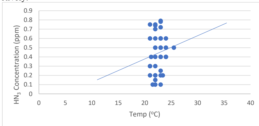
Figure 4: Correlation plot between ammonia ( \text{NH}_3 ) concentration levels and temperature (T)
