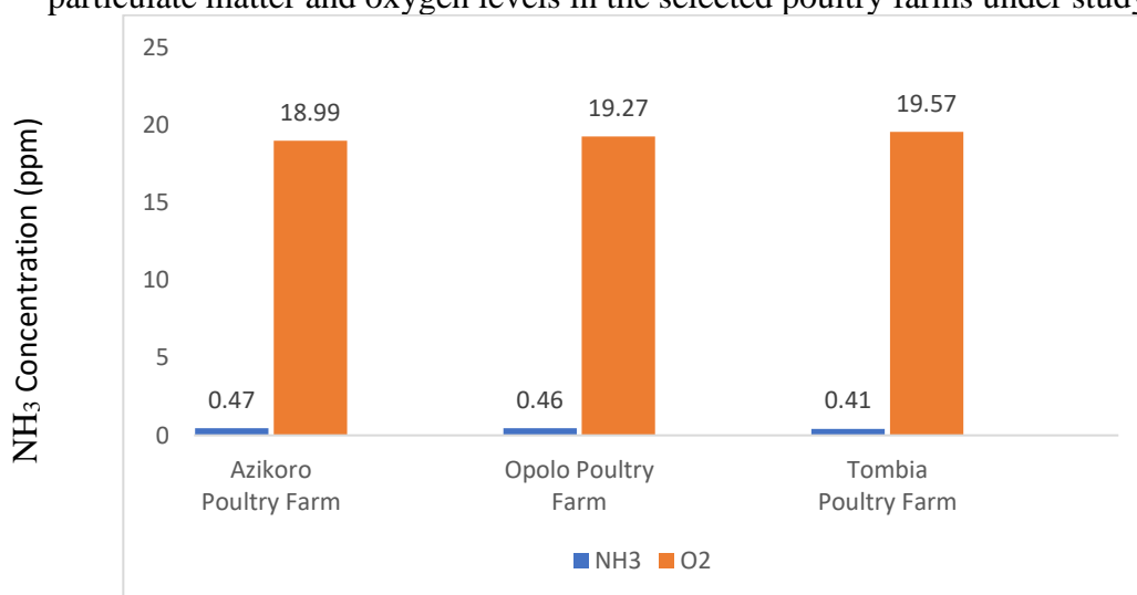
Figure 1: Concentration levels of ammonia ( \text{NH}_3 ) and oxygen ( \text{O}_2 ) in the selected poultry farms
