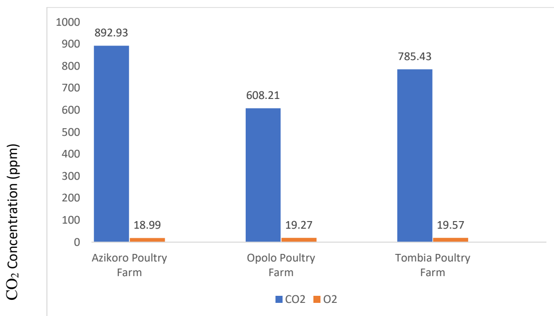
Figure 2: Concentration levels of carbon dioxide (CO 2 ) and Oxygen (O 2 ) in the selected poultry farms
